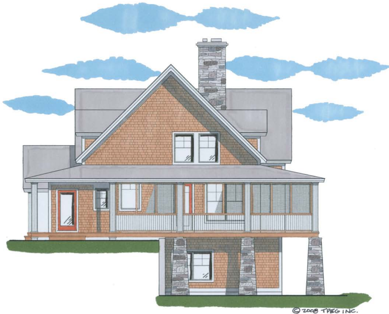
SIDE ELEVATION
