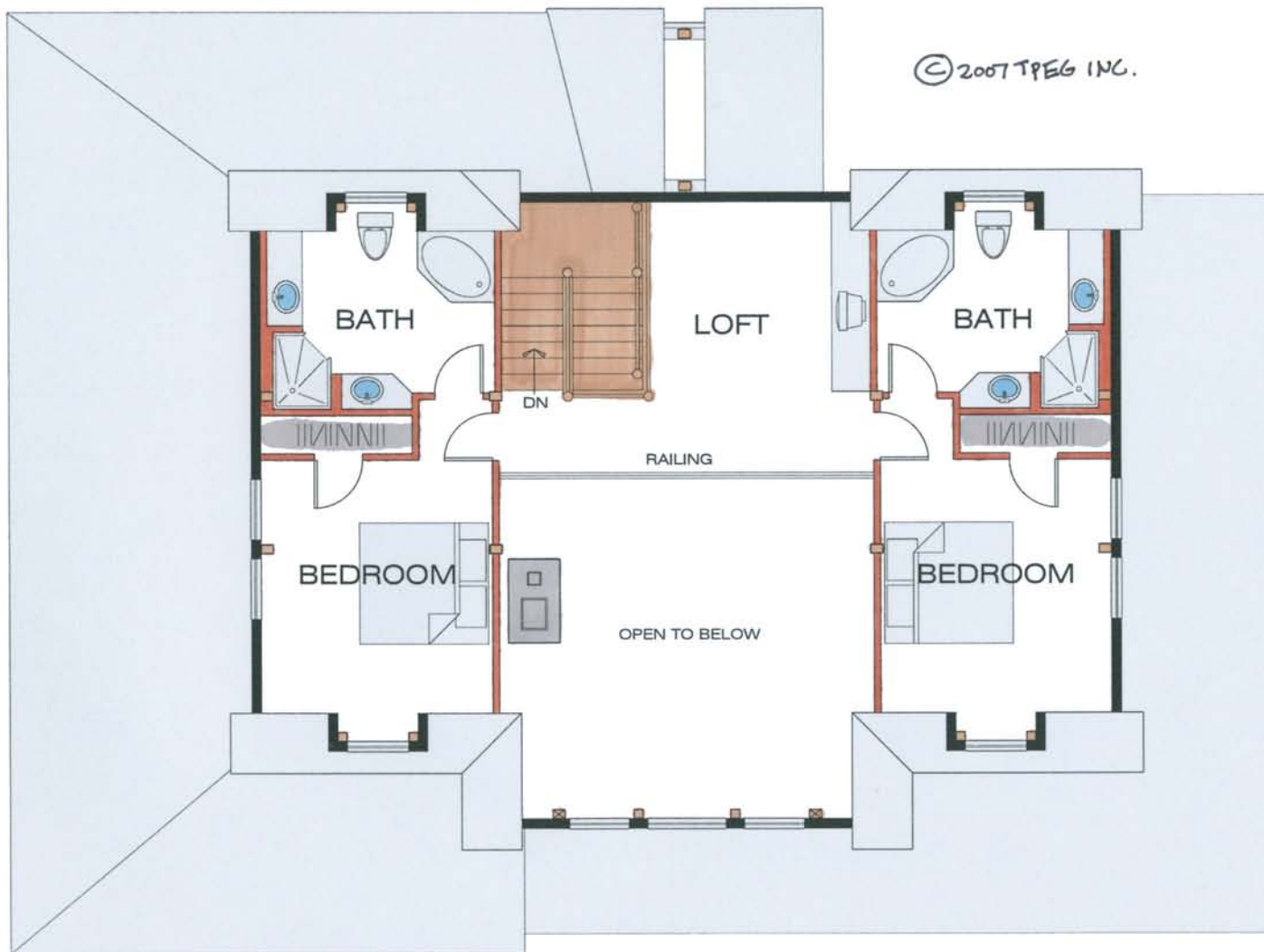
SECOND FLOOR PLAN 904 SQ. FEET
