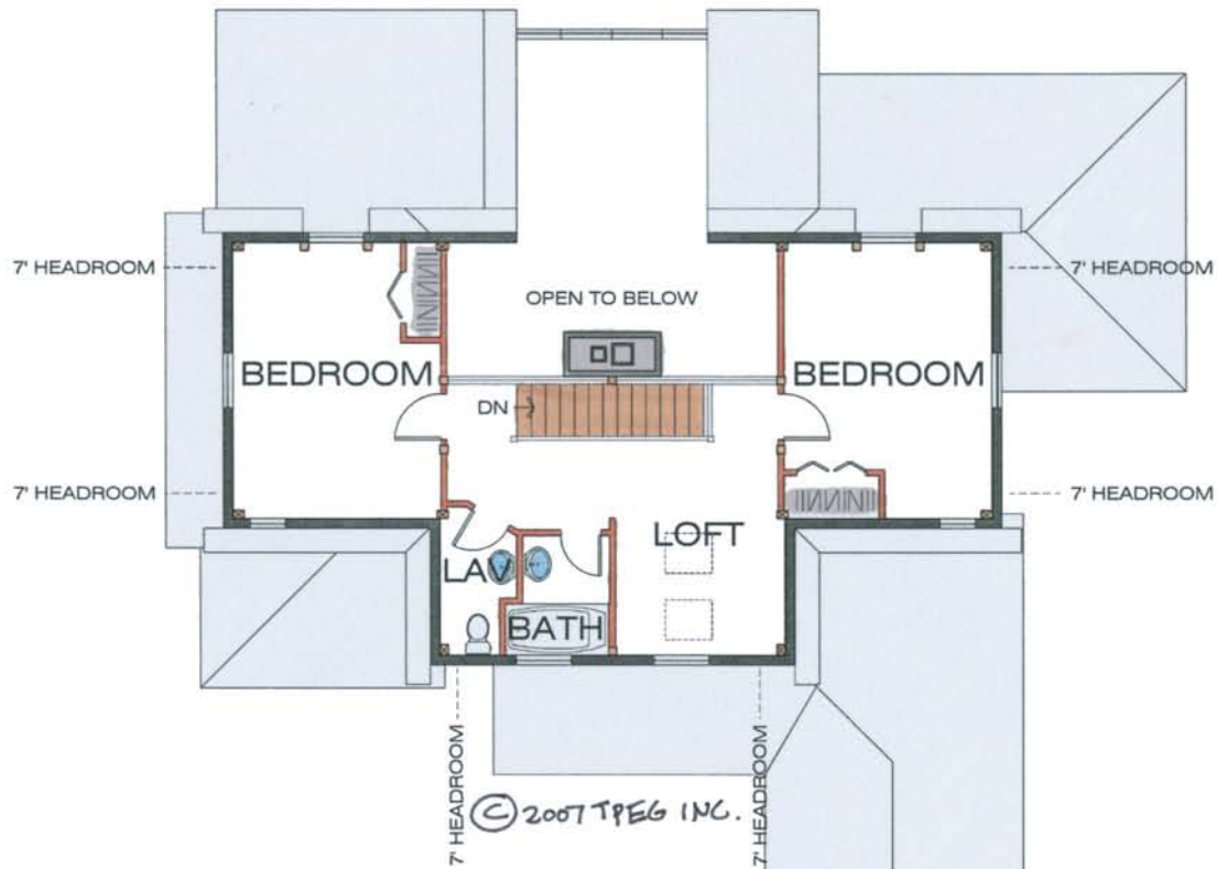
SECOND FLOOR PLAN 1084 SQ. FEET
