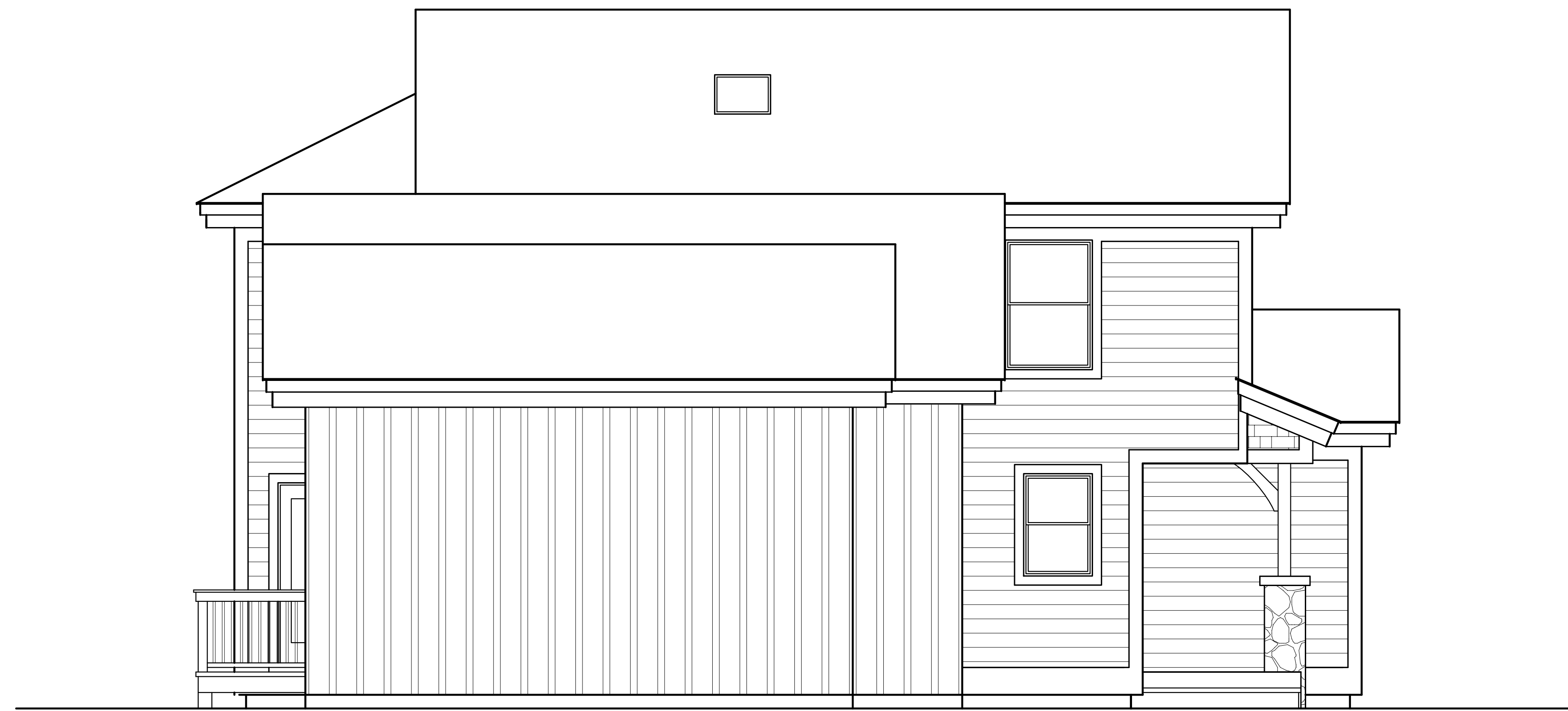
LEFT ELEVATION
