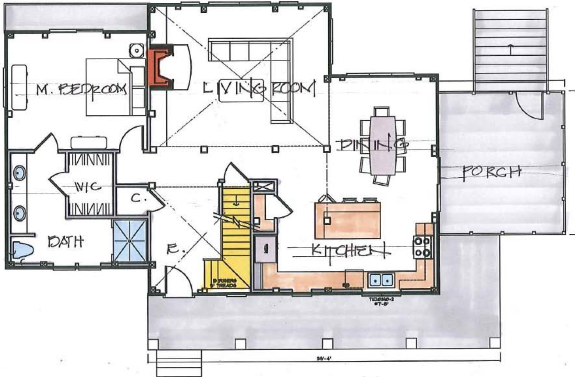
FIRST FLOOR 1344 SQ. FEET
