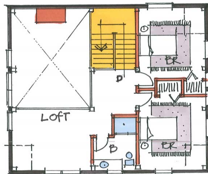
Second Floor - 715 sf
